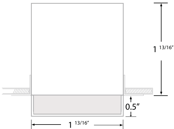
Channel Profile: 0.5 DP Option (Direct)
