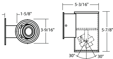
WD1340J - 4" ROUND
