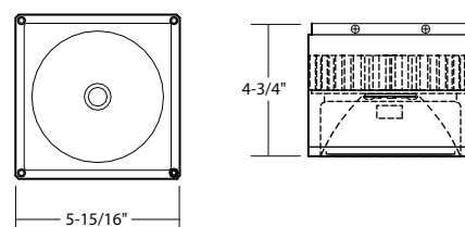
DLQ360 - 6" SQUARE
