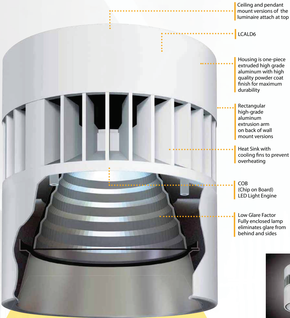
LCALD6EM Lumen Cannon 6" integral emergency option is available. See page 8 for ordering.
