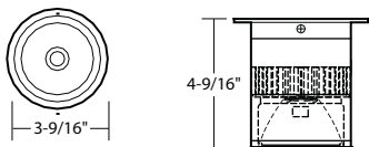
DL340 - 4" ROUND
