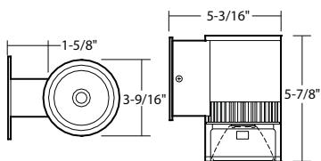
WD1340 - 4" ROUND
