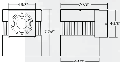
LWMLD6 - 6" Wall Mount
