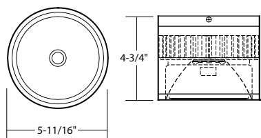
DL360 - 6" ROUND
