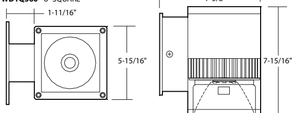
WD1Q360 - 6" SQUARE
