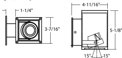
WD1Q340J - 4" SQUARE
