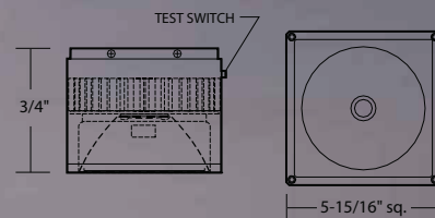
DLQ360EM - 6" EMERGENCY DOWNLIGHT
