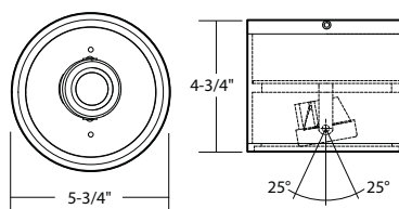
DL360J - 6" ROUND ADJUSTABLE
