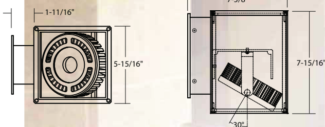
WD1Q360J - 6" SQUARE
