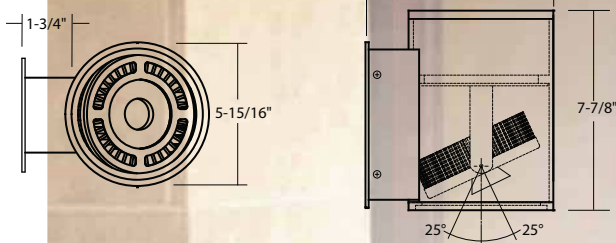
WD1360J - 6" ROUND
