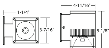
WD1Q340 - 4" SQUARE
