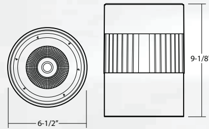
LCALD6X11 - 6" Ceiling/Pendant Mount
