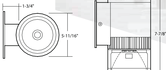
WD1Q360 - 6" SQUARE
