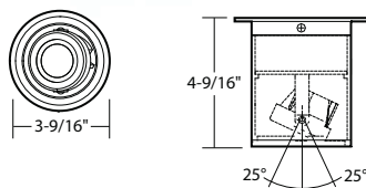
DL360J - 6" ROUND ADJUSTABLE
